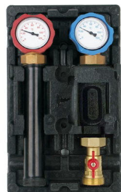
Item No:8100 Direct Circulation unit
